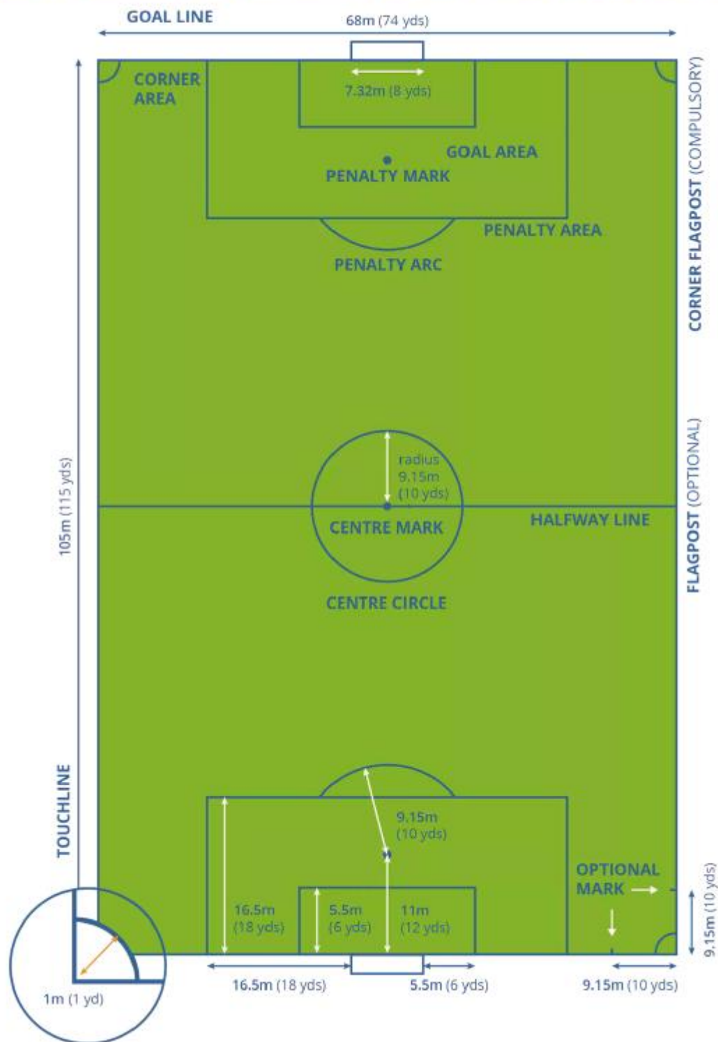
Layout- Football Field of play dimensions and pitch markings as per FIFA guidelines
