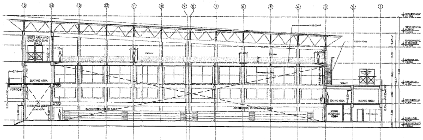
SECTION @Z-Z'
